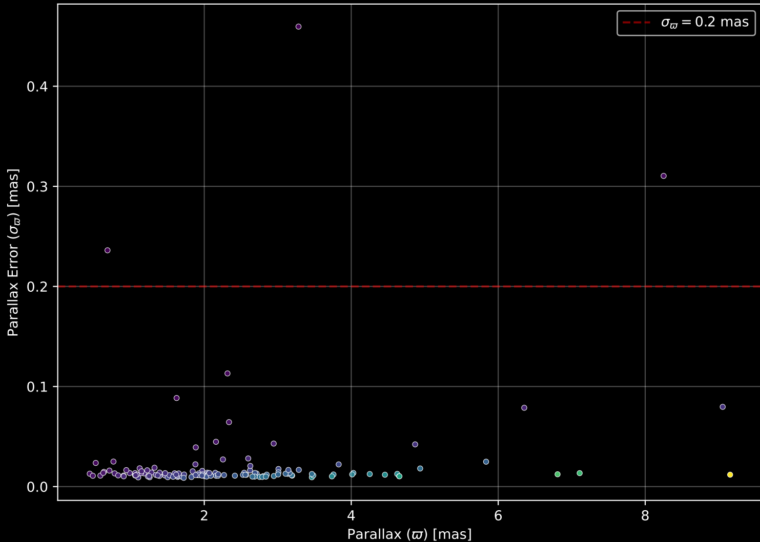
GALAH DR4 Field: [7178] Parallax Quality (n= 128)
