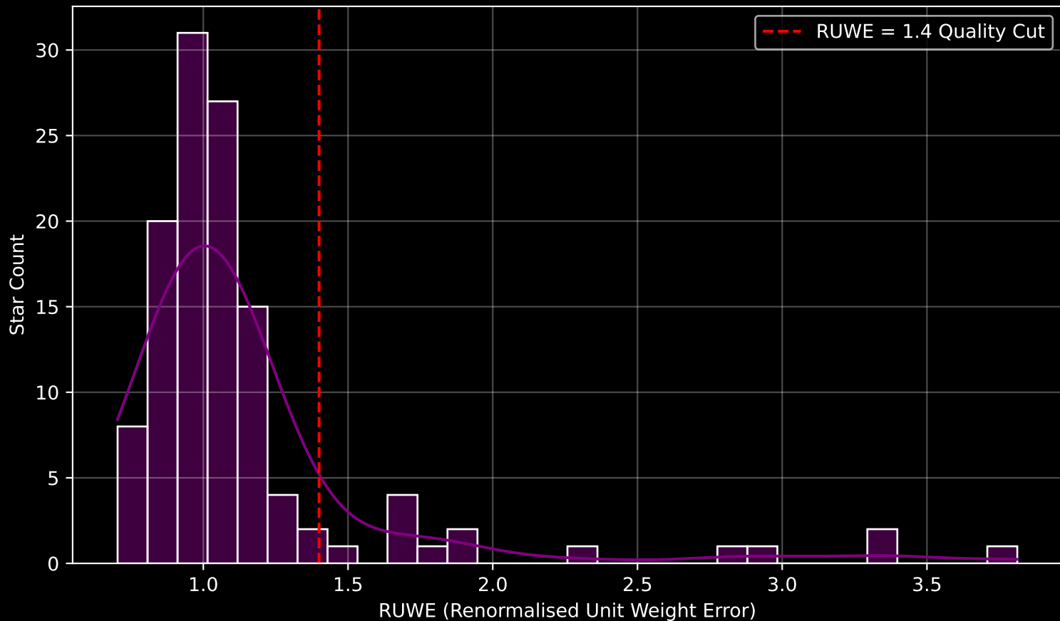
GALAH DR4 Field [7178] RUWE Distribution (n= 121)
