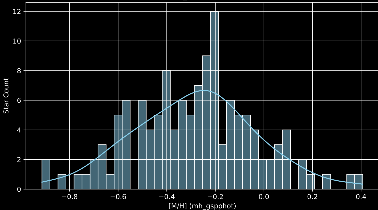
GALAH DR4 Field: [7178] [M/H] (mh_gspphot) (n= 128)
