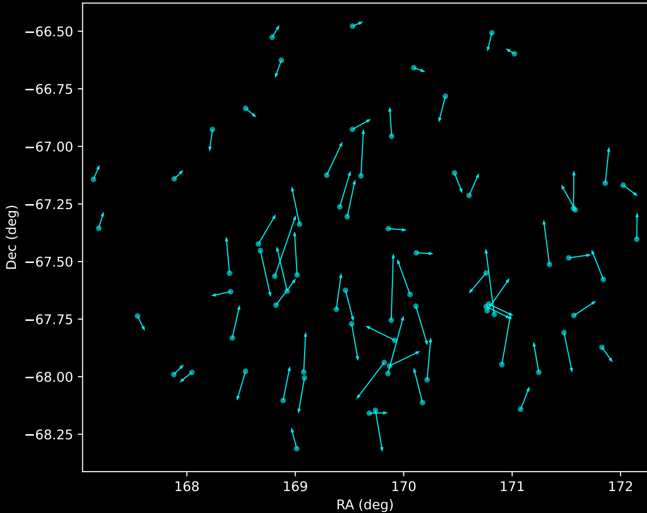
GALAH DR4 Noise Stream Proper Motion Vectors (n=73)
