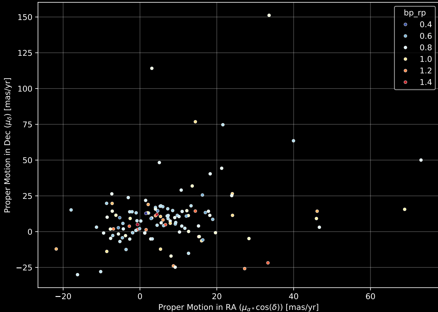
GALAH DR4 Field: [7178] Proper Motion Diagram (n= 128)
