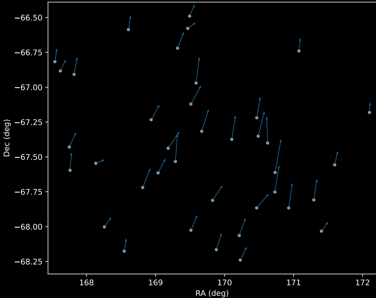
GALAH DR4 Cluster 0 Proper Motion Vectors (n=38)
