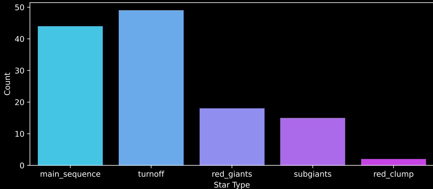
GALAH DR4 Field: [7178] Count plot of Star Type
